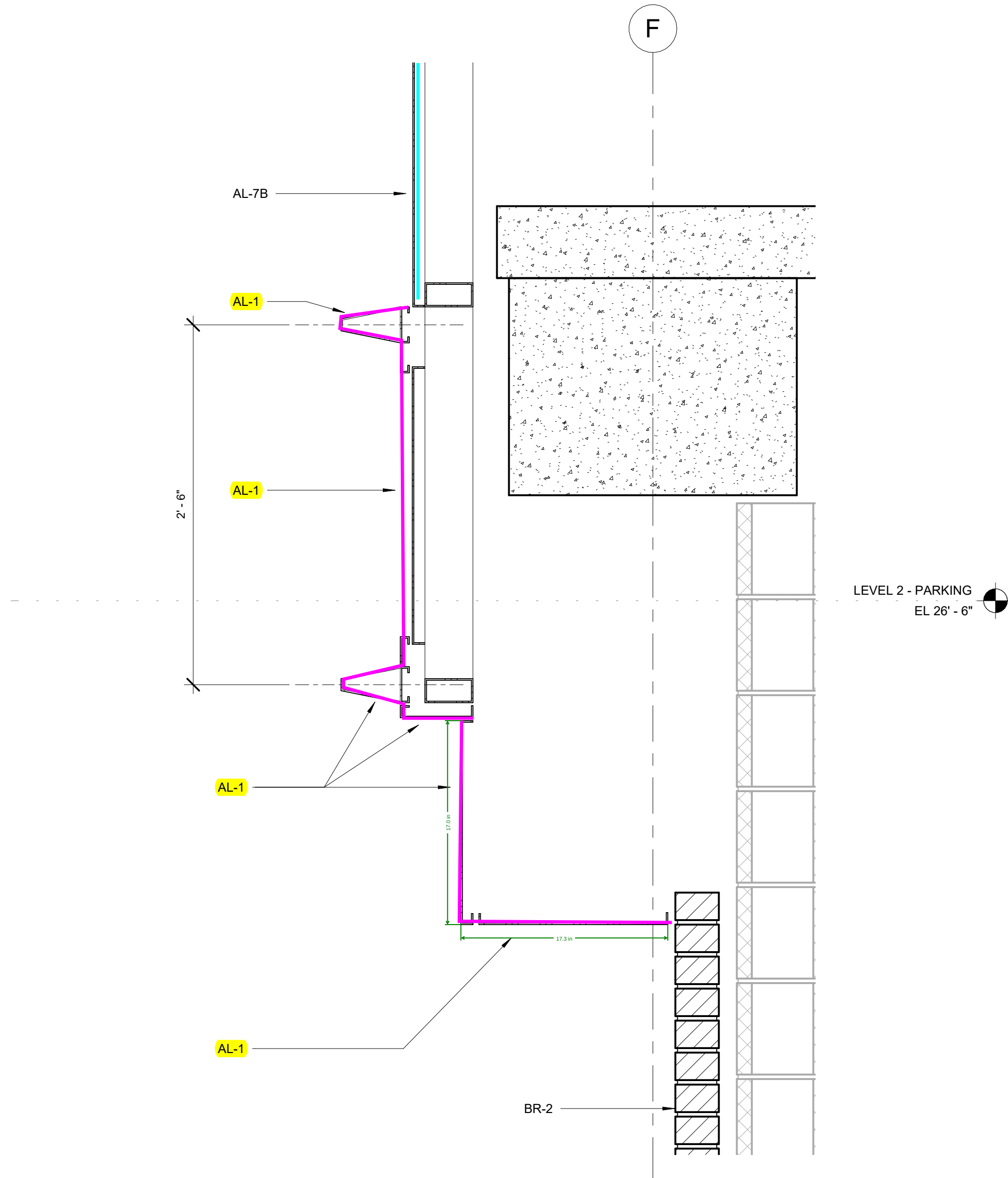
2 TERRACOTTA METAL PANEL DETAIL - SECTION 1 1/2" = 1'-0"
