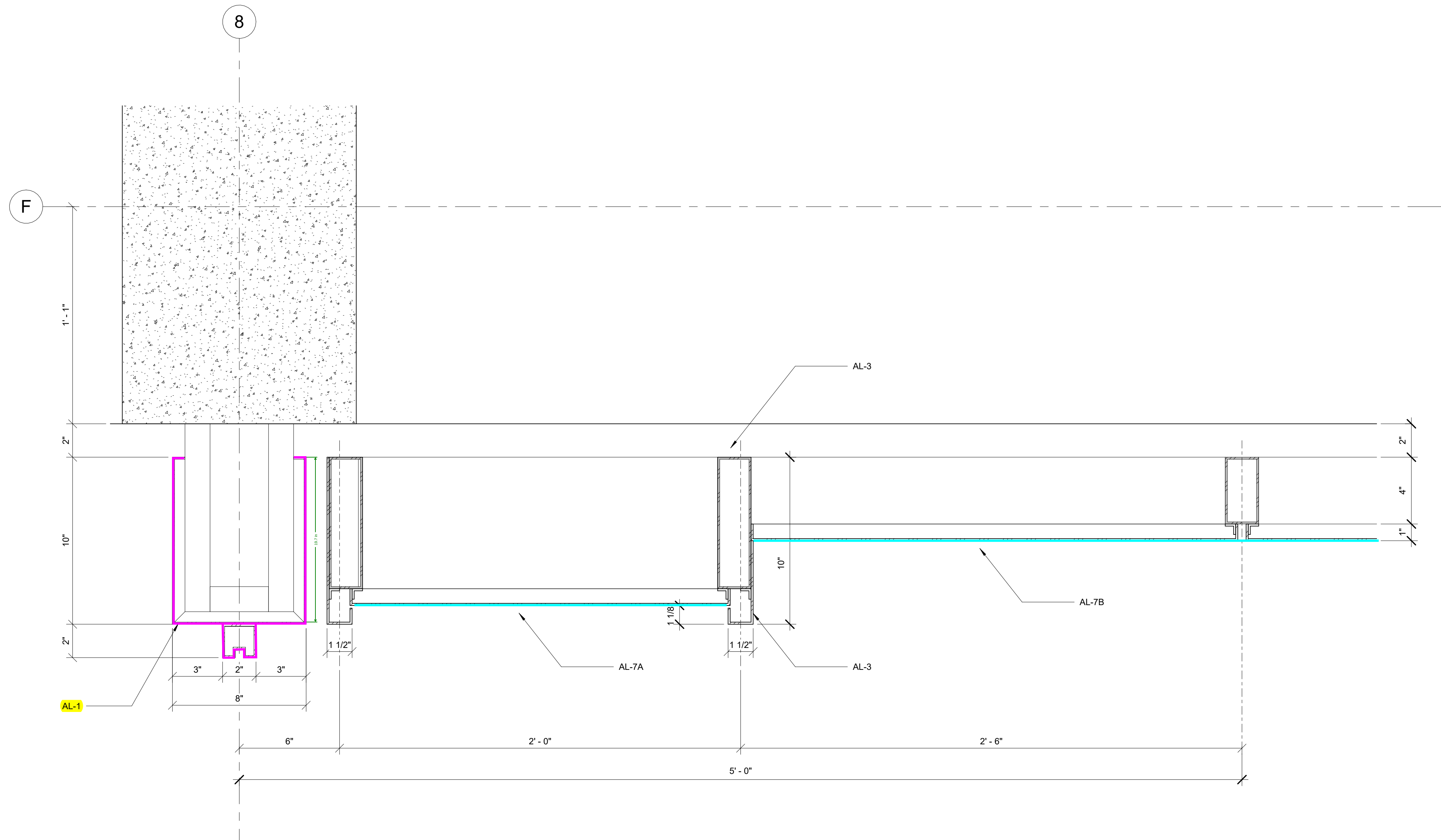
3 GARAGE PLAN DETAIL 3" = 1'-0"
